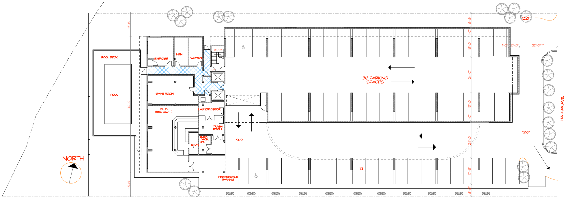
1ST (GROUND) FLOOR PLAN ——— 1"=20'-0"
