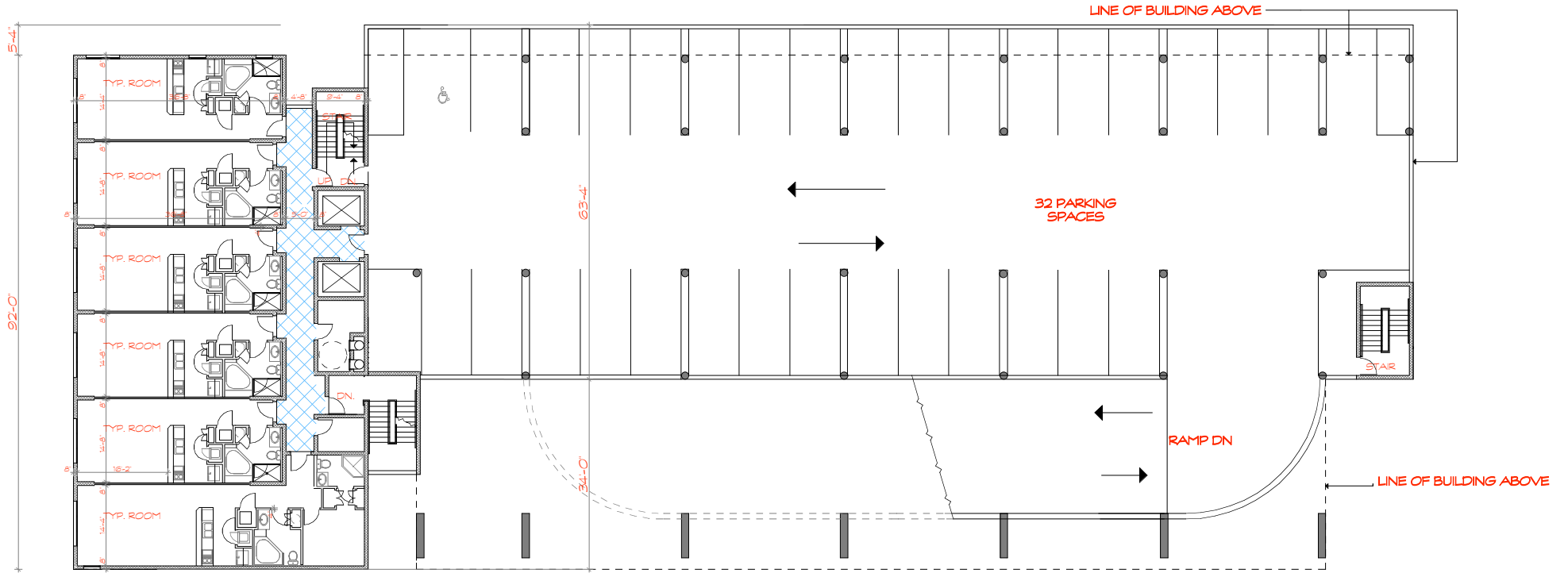
5TH FLOOR PLAN-(6 UNITS)-----3/32'
