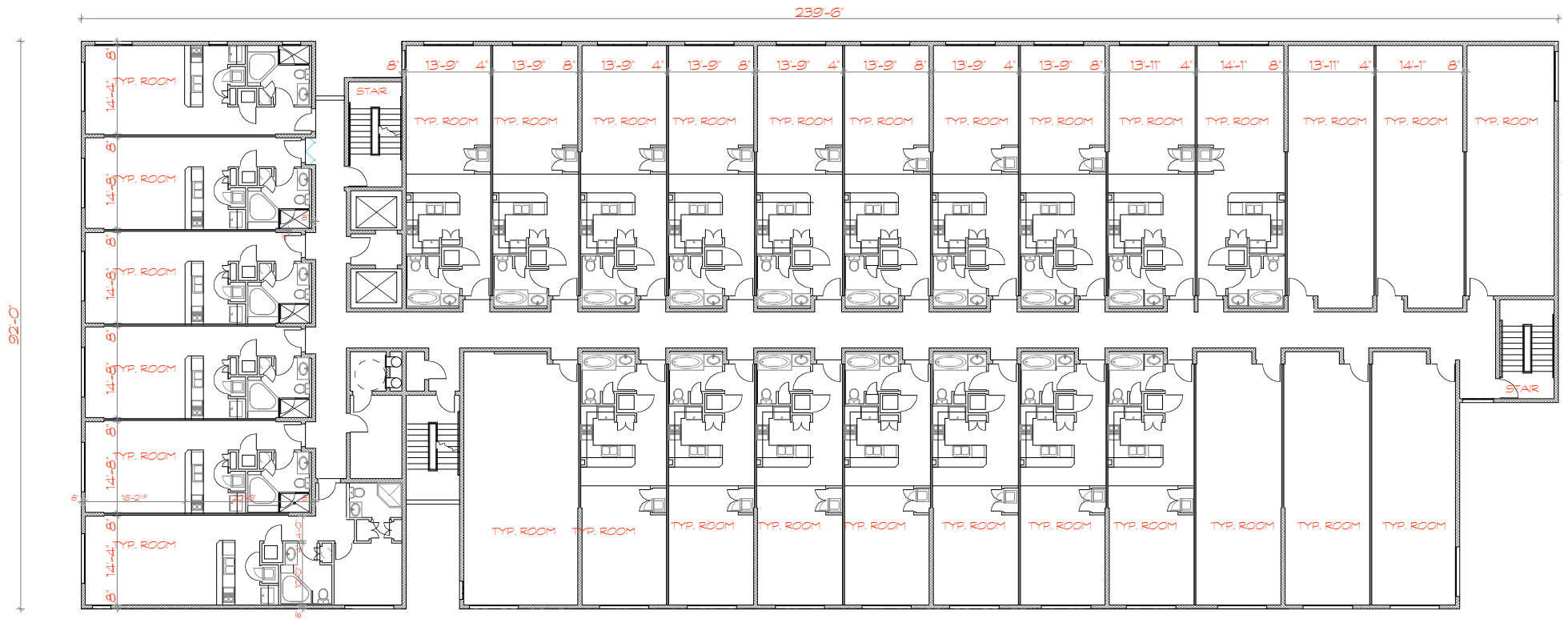
6TH, THRU 9TH FLOOR PLANS--(120 UNITS)-----1/8"
